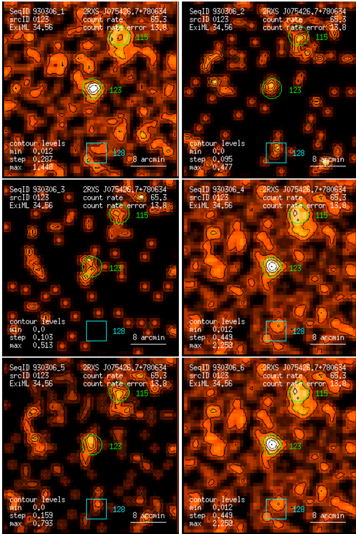
Figure 123: RASS 930306: detection 0123: band rate images, Gaussian filter: (1) PSPC channels 11 – 41, (2) 52 – 90, (3) 91 – 201, (4) 11 – 235, (5) 52 – 201, (6) 11 – 201. Broad band rates in counts/ks. Band rate contour levels in counts/ks/arcmin 2 .
