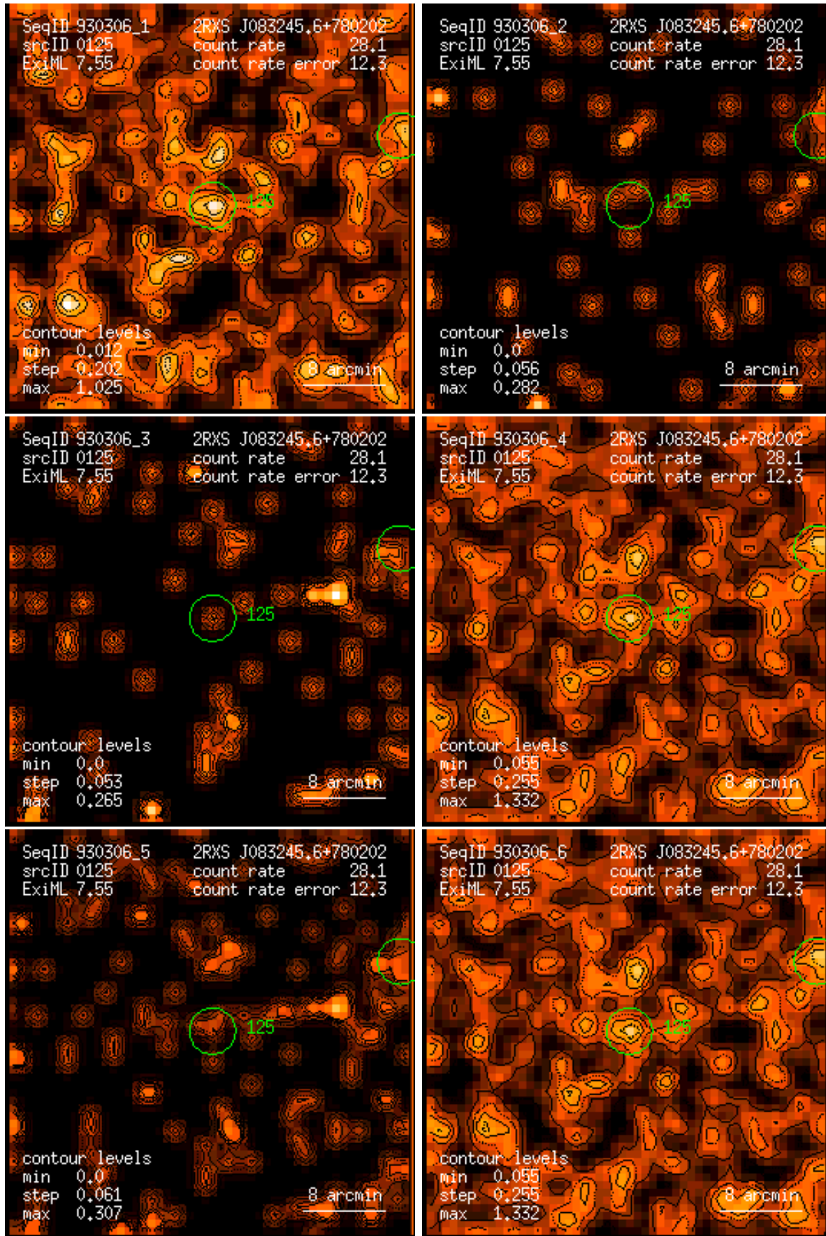
Figure 125: RASS 930306: detection 0125: band rate images, Gaussian filter: (1) PSPC channels 11 – 41, (2) 52 – 90, (3) 91 – 201, (4) 11 – 235, (5) 52 – 201, (6) 11 – 201. Broad band rates in counts/ks. Band rate contour levels in counts/ks/arcmin 2 .
