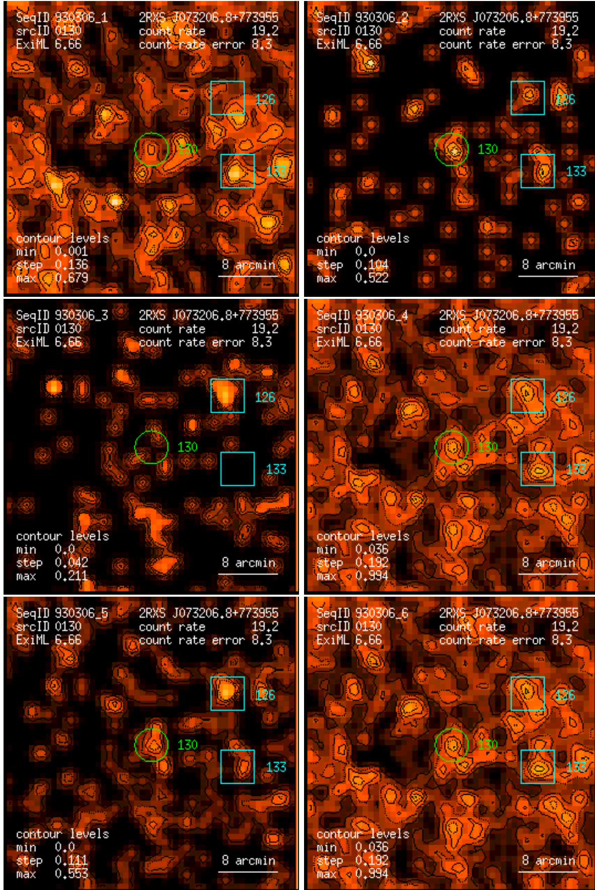
Figure 130: RASS 930306: detection 0130: band rate images, Gaussian filter: (1) PSPC channels 11 – 41, (2) 52 – 90, (3) 91 – 201, (4) 11 – 235, (5) 52 – 201, (6) 11 – 201. Broad band rates in counts/ks. Band rate contour levels in counts/ks/arcmin 2 .
