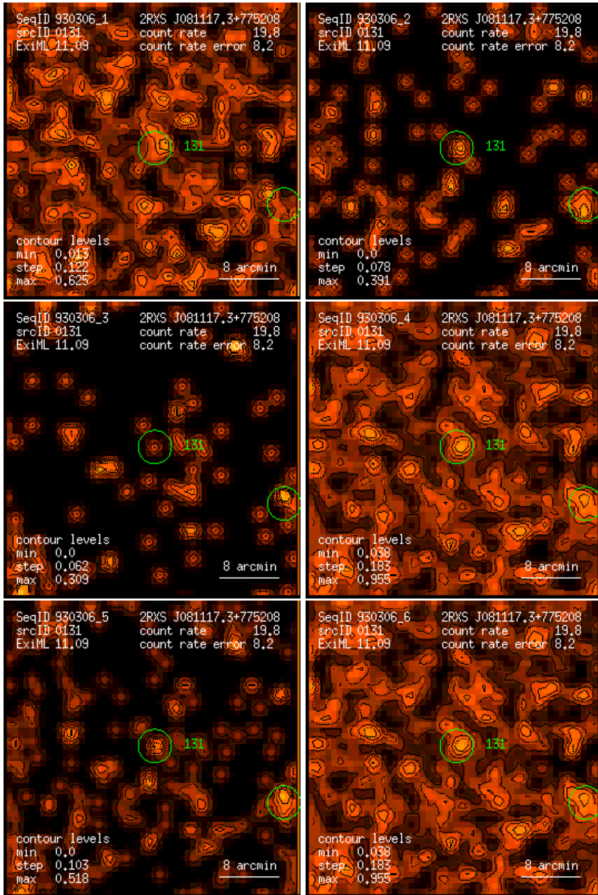
Figure 131: RASS 930306: detection 0131: band rate images, Gaussian filter: (1) PSPC channels 11 – 41, (2) 52 – 90, (3) 91 – 201, (4) 11 – 235, (5) 52 – 201, (6) 11 – 201. Broad band rates in counts/ks. Band rate contour levels in counts/ks/arcmin 2 .
