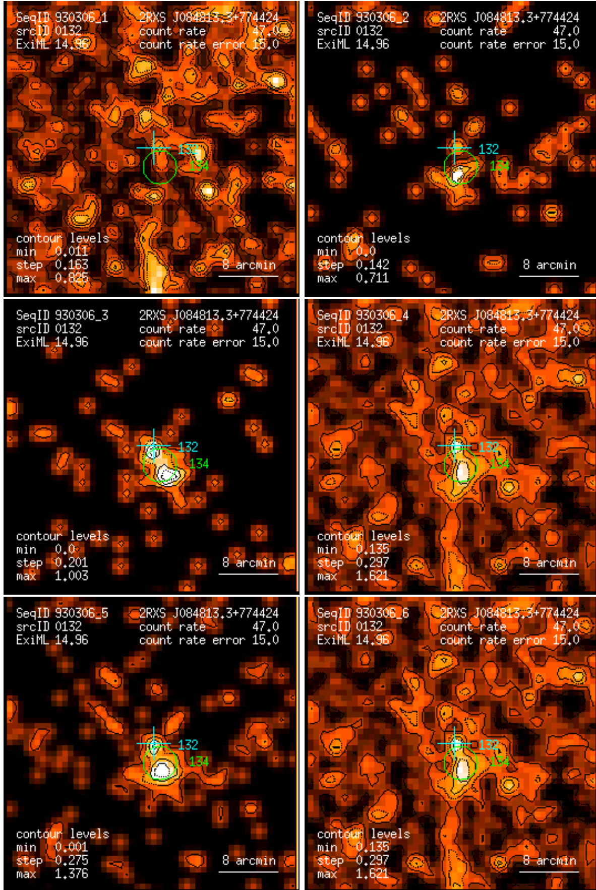
Figure 132: RASS 930306: detection 0132: band rate images, Gaussian filter: (1) PSPC channels 11 – 41, (2) 52 – 90, (3) 91 – 201, (4) 11 – 235, (5) 52 – 201, (6) 11 – 201. Broad band rates in counts/ks. Band rate contour levels in counts/ks/arcmin 2 .
