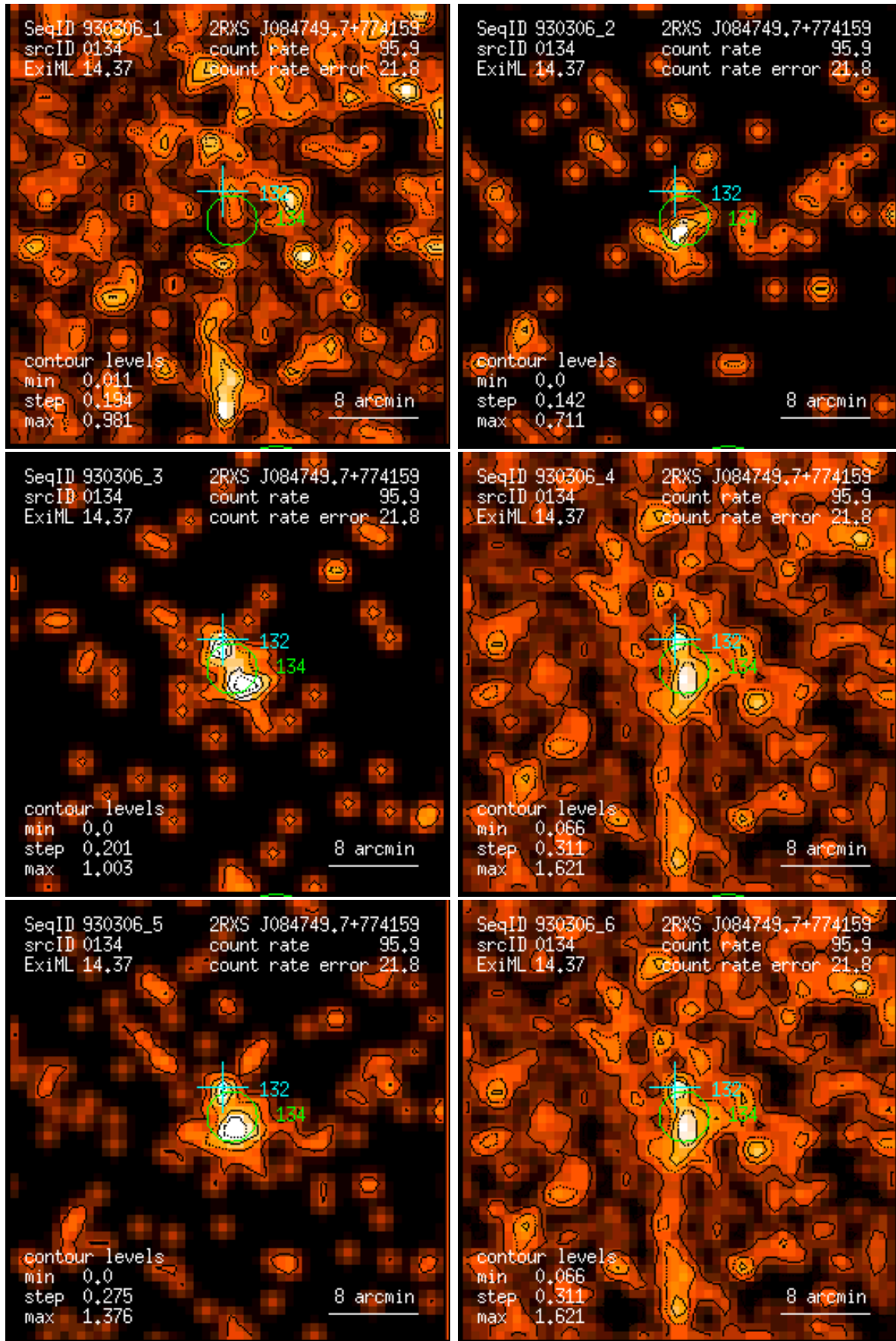
Figure 134: RASS 930306: detection 0134: band rate images, Gaussian filter: (1) PSPC channels 11 – 41, (2) 52 – 90, (3) 91 – 201, (4) 11 – 235, (5) 52 – 201, (6) 11 – 201. Broad band rates in counts/ks. Band rate contour levels in counts/ks/arcmin 2 .
