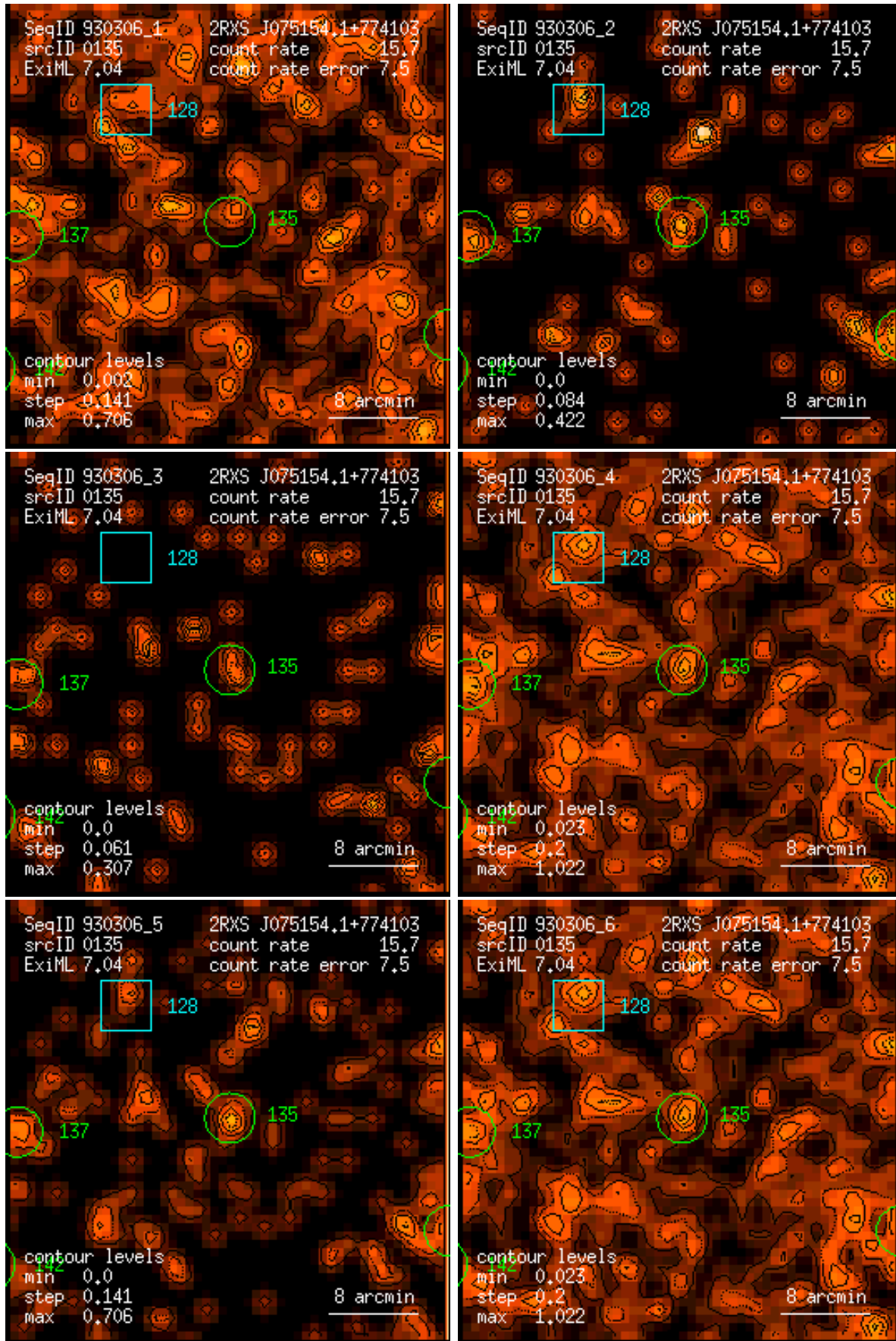
Figure 135: RASS 930306: detection 0135: band rate images, Gaussian filter: (1) PSPC channels 11 – 41, (2) 52 – 90, (3) 91 – 201, (4) 11 – 235, (5) 52 – 201, (6) 11 – 201. Broad band rates in counts/ks. Band rate contour levels in counts/ks/arcmin 2 .
