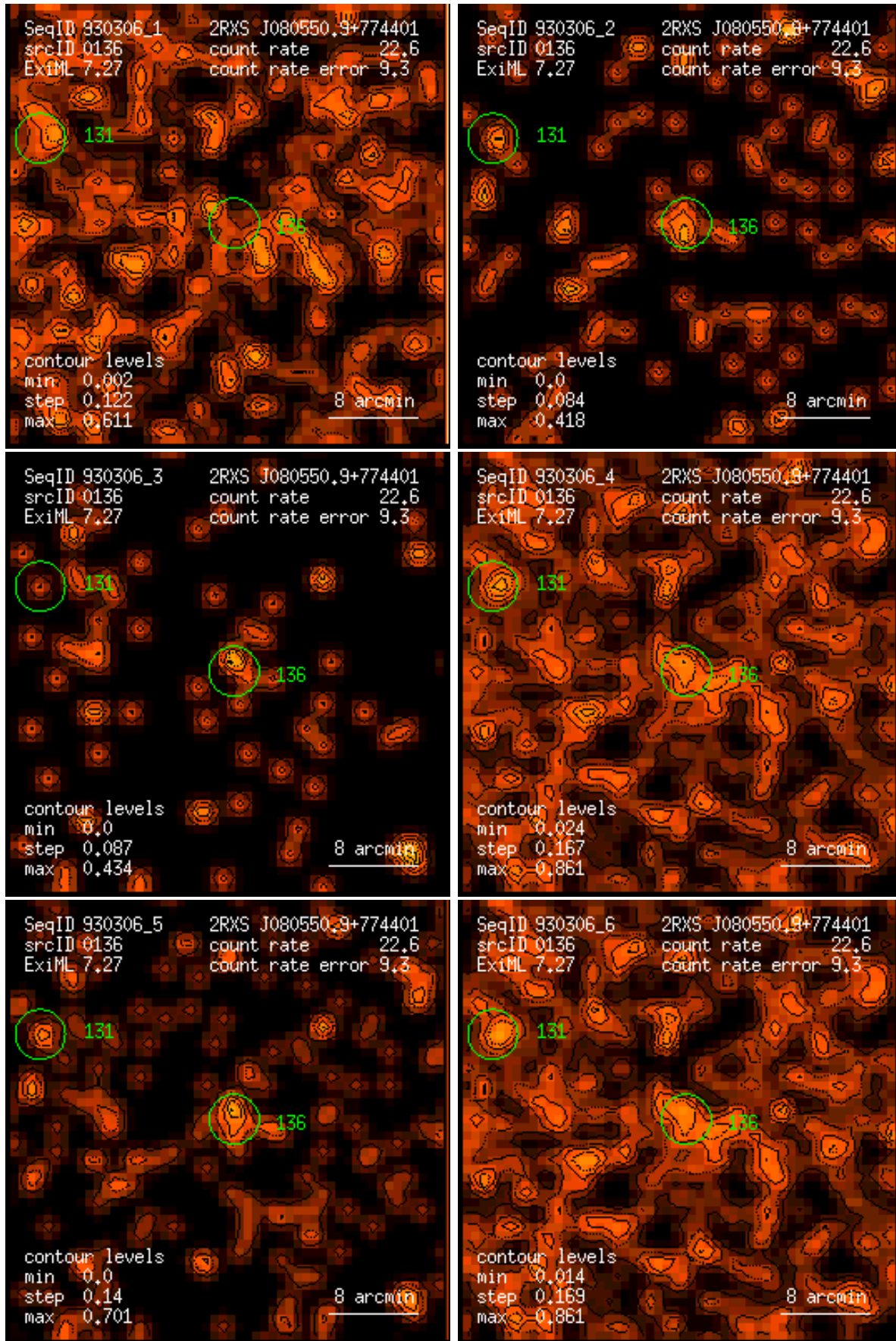
Figure 136: RASS 930306: detection 0136: band rate images, Gaussian filter: (1) PSPC channels 11 – 41, (2) 52 – 90, (3) 91 – 201, (4) 11 – 235, (5) 52 – 201, (6) 11 – 201. Broad band rates in counts/ks. Band rate contour levels in counts/ks/arcmin 2 .
