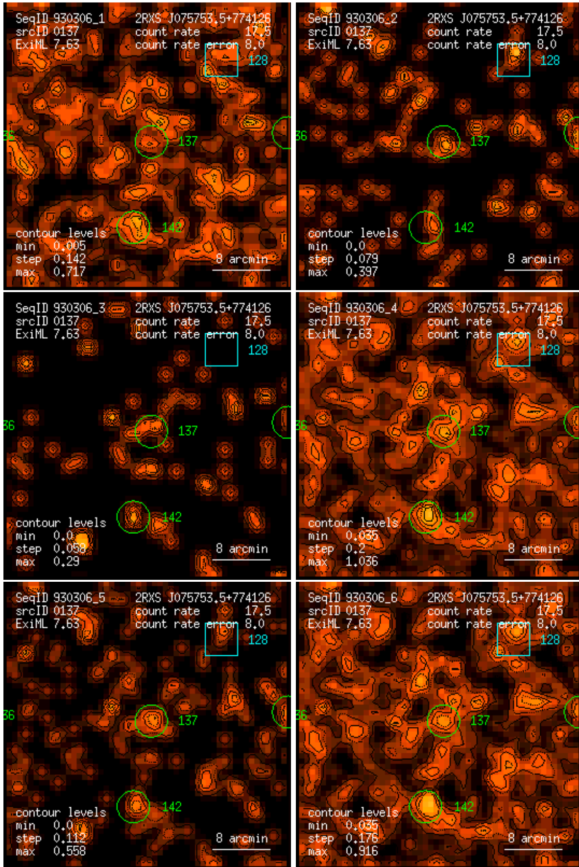
Figure 137: RASS 930306: detection 0137: band rate images, Gaussian filter: (1) PSPC channels 11 – 41, (2) 52 – 90, (3) 91 – 201, (4) 11 – 235, (5) 52 – 201, (6) 11 – 201. Broad band rates in counts/ks. Band rate contour levels in counts/ks/arcmin 2 .
