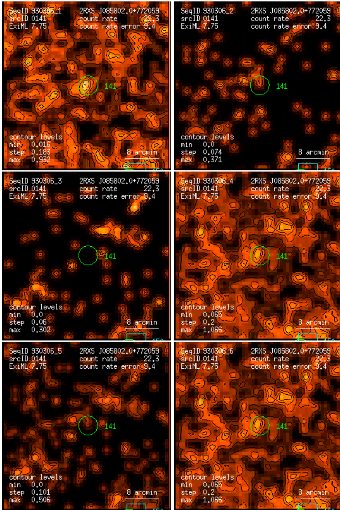
Figure 141: RASS 930306: detection 0141: band rate images, Gaussian filter: (1) PSPC channels 11 – 41, (2) 52 – 90, (3) 91 – 201, (4) 11 – 235, (5) 52 – 201, (6) 11 – 201. Broad band rates in counts/ks. Band rate contour levels in counts/ks/arcmin 2 .
