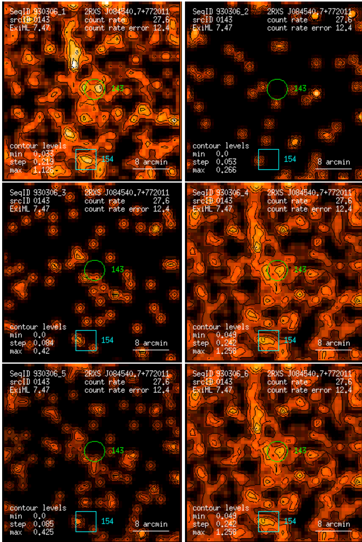
Figure 143: RASS 930306: detection 0143: band rate images, Gaussian filter: (1) PSPC channels 11 – 41, (2) 52 – 90, (3) 91 – 201, (4) 11 – 235, (5) 52 – 201, (6) 11 – 201. Broad band rates in counts/ks. Band rate contour levels in counts/ks/arcmin 2 .
