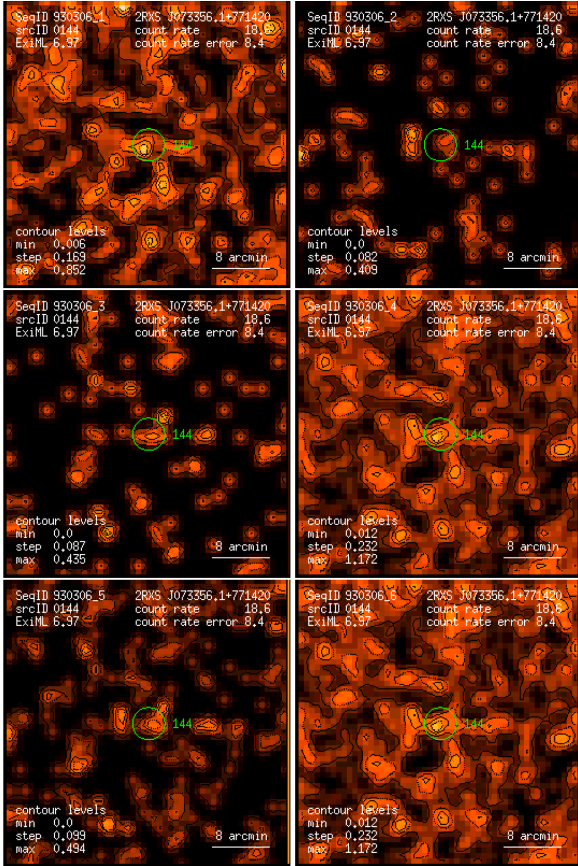
Figure 144: RASS 930306: detection 0144: band rate images, Gaussian filter: (1) PSPC channels 11 – 41, (2) 52 – 90, (3) 91 – 201, (4) 11 – 235, (5) 52 – 201, (6) 11 – 201. Broad band rates in counts/ks. Band rate contour levels in counts/ks/arcmin 2 .
