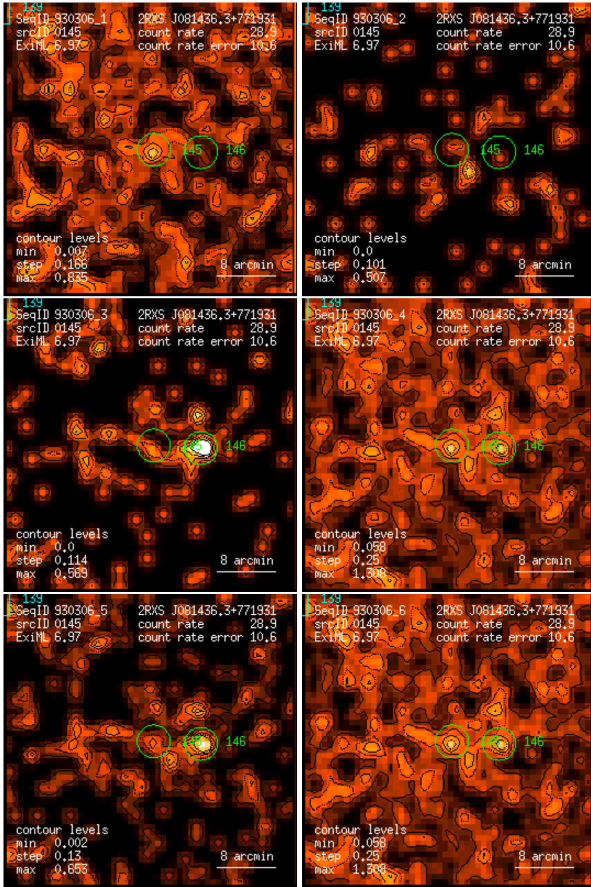
Figure 145: RASS 930306: detection 0145: band rate images, Gaussian filter: (1) PSPC channels 11 – 41, (2) 52 – 90, (3) 91 – 201, (4) 11 – 235, (5) 52 – 201, (6) 11 – 201. Broad band rates in counts/ks. Band rate contour levels in counts/ks/arcmin 2 .
