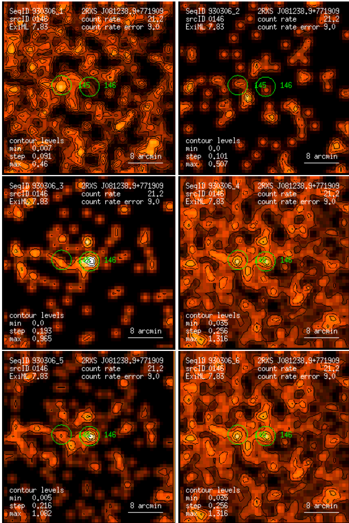
Figure 146: RASS 930306: detection 0146: band rate images, Gaussian filter: (1) PSPC channels 11 – 41, (2) 52 – 90, (3) 91 – 201, (4) 11 – 235, (5) 52 – 201, (6) 11 – 201. Broad band rates in counts/ks. Band rate contour levels in counts/ks/arcmin 2 .
