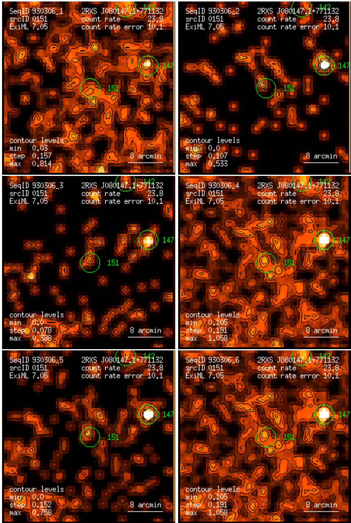
Figure 151: RASS 930306: detection 0151: band rate images, Gaussian filter: (1) PSPC channels 11 – 41, (2) 52 – 90, (3) 91 – 201, (4) 11 – 235, (5) 52 – 201, (6) 11 – 201. Broad band rates in counts/ks. Band rate contour levels in counts/ks/arcmin 2 .
