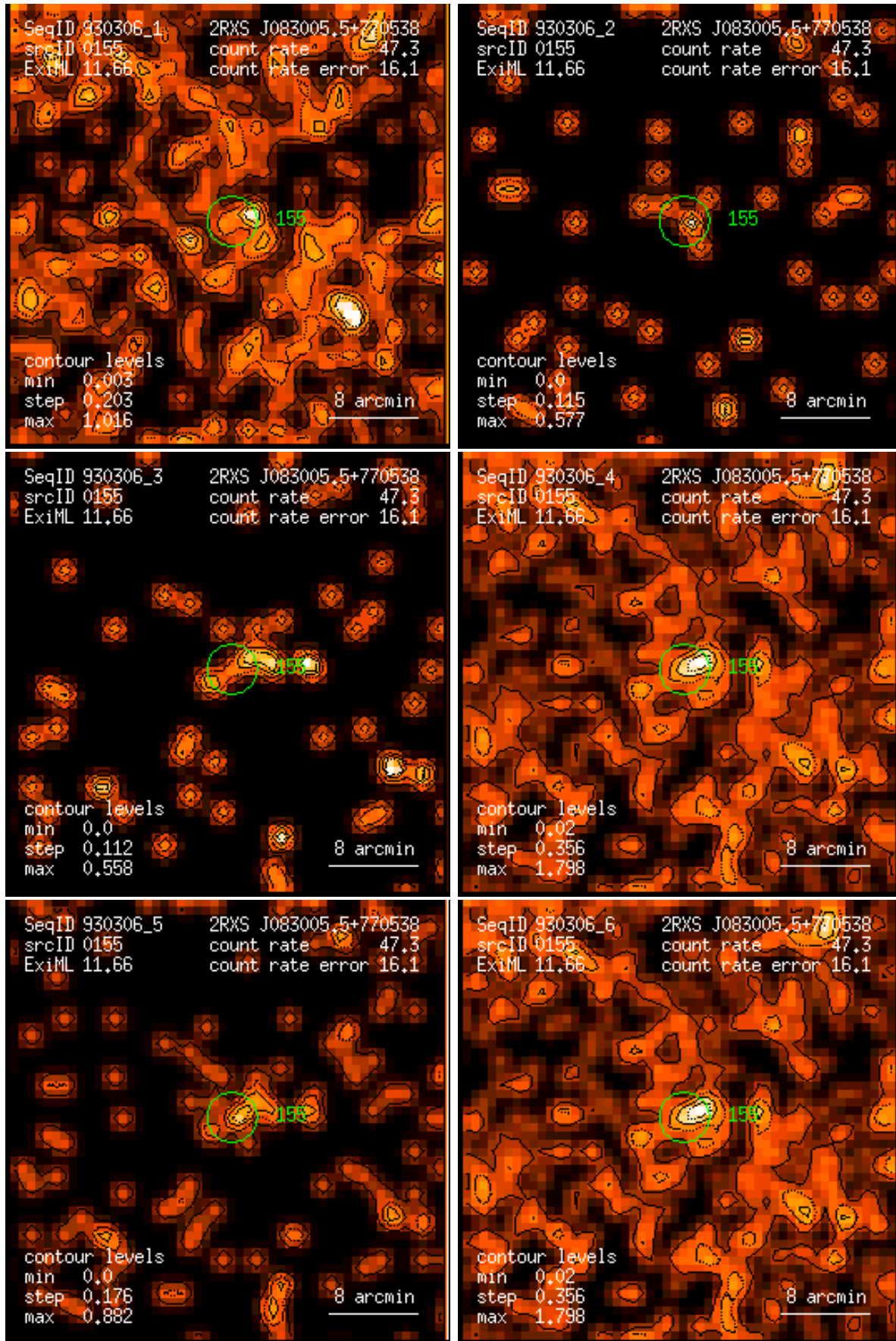
Figure 155: RASS 930306: detection 0155: band rate images, Gaussian filter: (1) PSPC channels 11 – 41, (2) 52 – 90, (3) 91 – 201, (4) 11 – 235, (5) 52 – 201, (6) 11 – 201. Broad band rates in counts/ks. Band rate contour levels in counts/ks/arcmin 2 .
