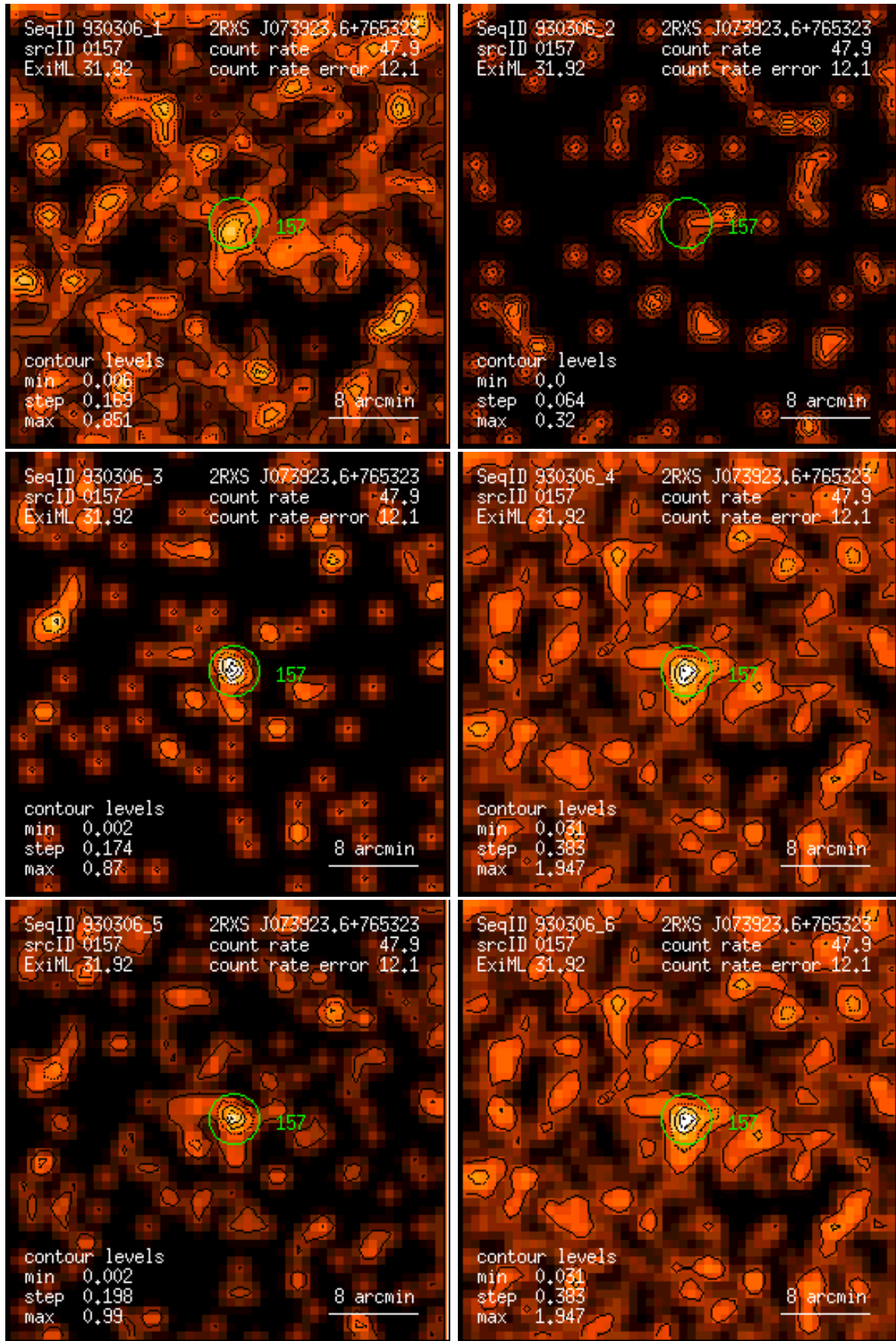
Figure 157: RASS 930306: detection 0157: band rate images, Gaussian filter: (1) PSPC channels 11 – 41, (2) 52 – 90, (3) 91 – 201, (4) 11 – 235, (5) 52 – 201, (6) 11 – 201. Broad band rates in counts/ks. Band rate contour levels in counts/ks/arcmin 2 .
