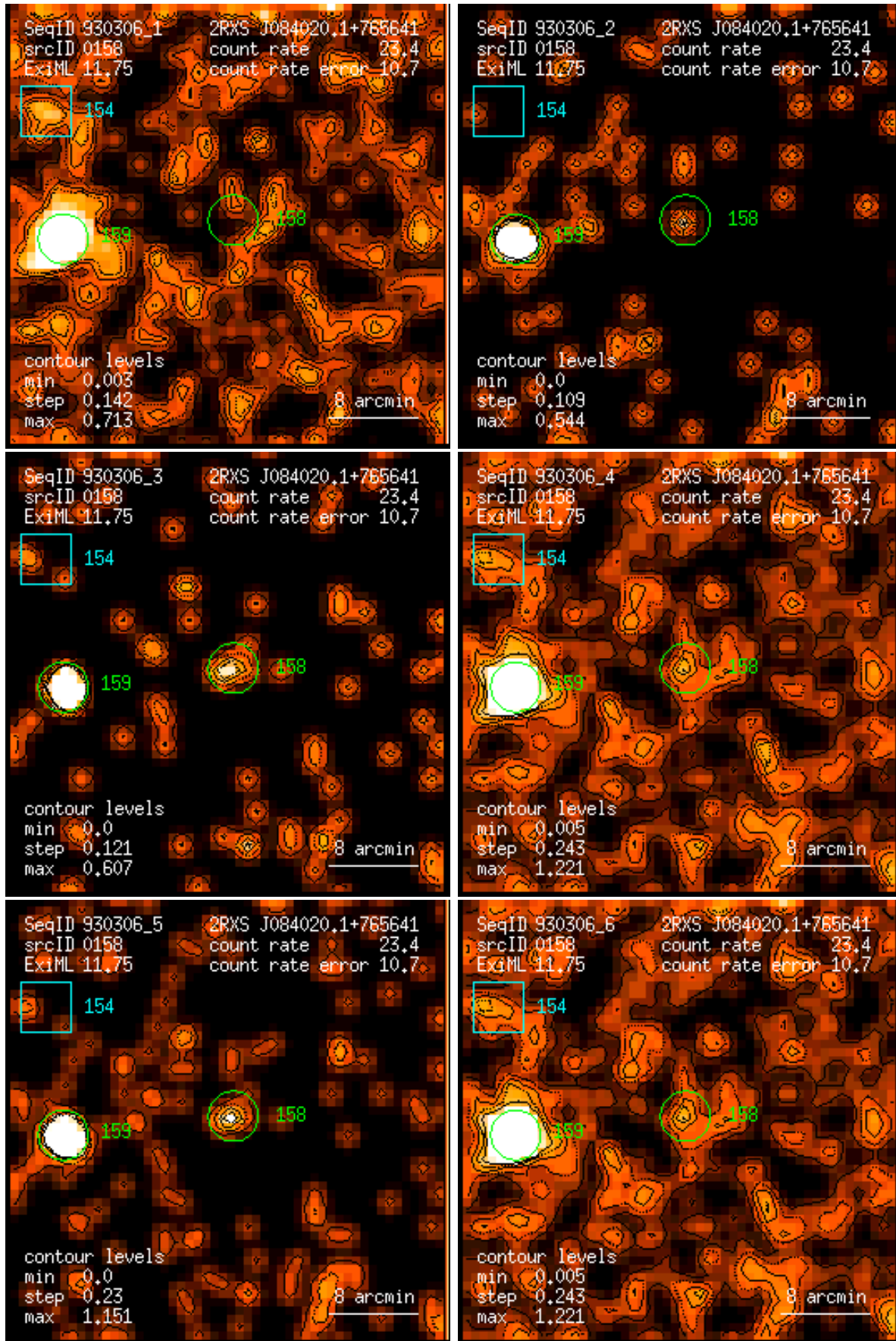
Figure 158: RASS 930306: detection 0158: band rate images, Gaussian filter: (1) PSPC channels 11 – 41, (2) 52 – 90, (3) 91 – 201, (4) 11 – 235, (5) 52 – 201, (6) 11 – 201. Broad band rates in counts/ks. Band rate contour levels in counts/ks/arcmin 2 .
