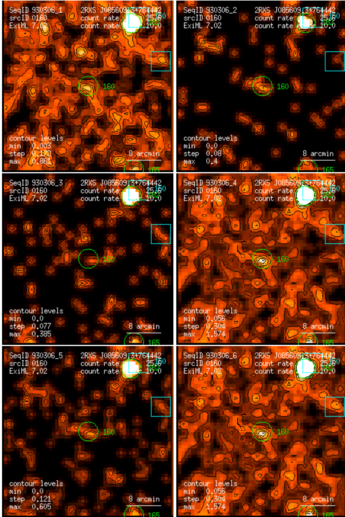
Figure 160: RASS 930306: detection 0160: band rate images, Gaussian filter: (1) PSPC channels 11 – 41, (2) 52 – 90, (3) 91 – 201, (4) 11 – 235, (5) 52 – 201, (6) 11 – 201. Broad band rates in counts/ks. Band rate contour levels in counts/ks/arcmin 2 .
