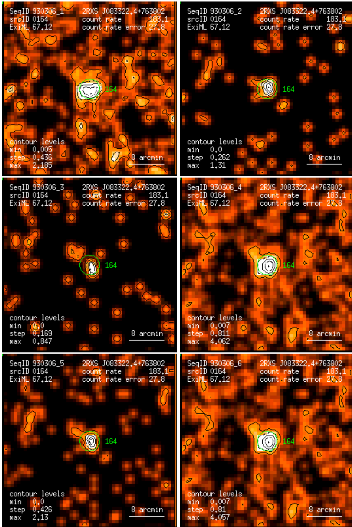
Figure 164: RASS 930306: detection 0164: band rate images, Gaussian filter: (1) PSPC channels 11 – 41, (2) 52 – 90, (3) 91 – 201, (4) 11 – 235, (5) 52 – 201, (6) 11 – 201. Broad band rates in counts/ks. Band rate contour levels in counts/ks/arcmin 2 .
