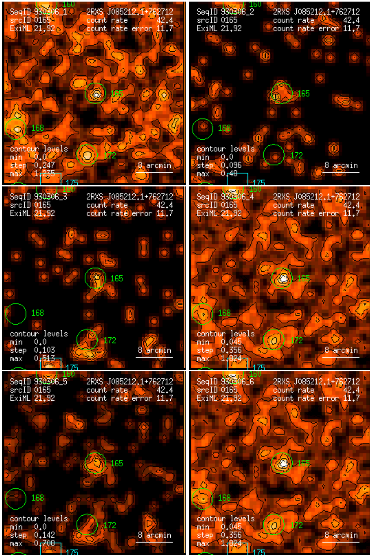
Figure 165: RASS 930306: detection 0165: band rate images, Gaussian filter: (1) PSPC channels 11 – 41, (2) 52 – 90, (3) 91 – 201, (4) 11 – 235, (5) 52 – 201, (6) 11 – 201. Broad band rates in counts/ks. Band rate contour levels in counts/ks/arcmin 2 .
