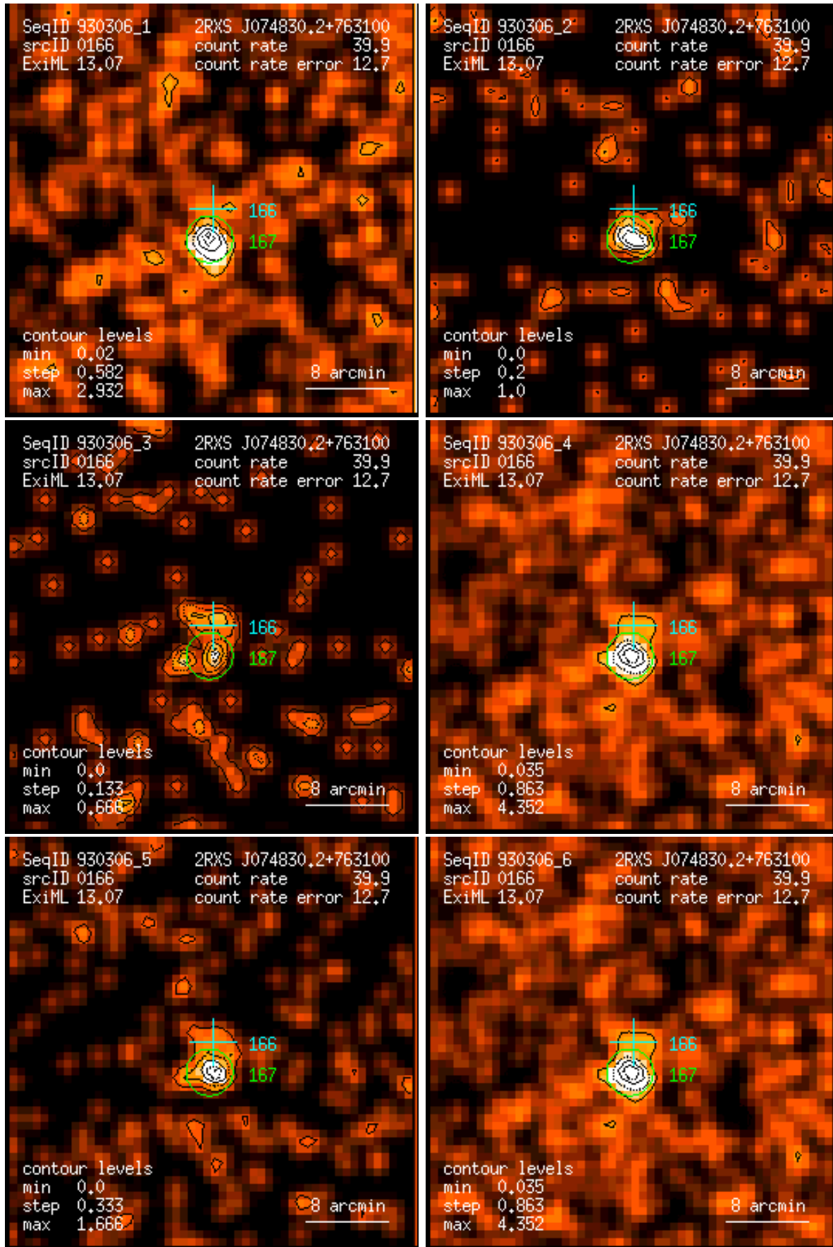
Figure 166: RASS 930306: detection 0166: band rate images, Gaussian filter: (1) PSPC channels 11 – 41, (2) 52 – 90, (3) 91 – 201, (4) 11 – 235, (5) 52 – 201, (6) 11 – 201. Broad band rates in counts/ks. Band rate contour levels in counts/ks/arcmin 2 .
