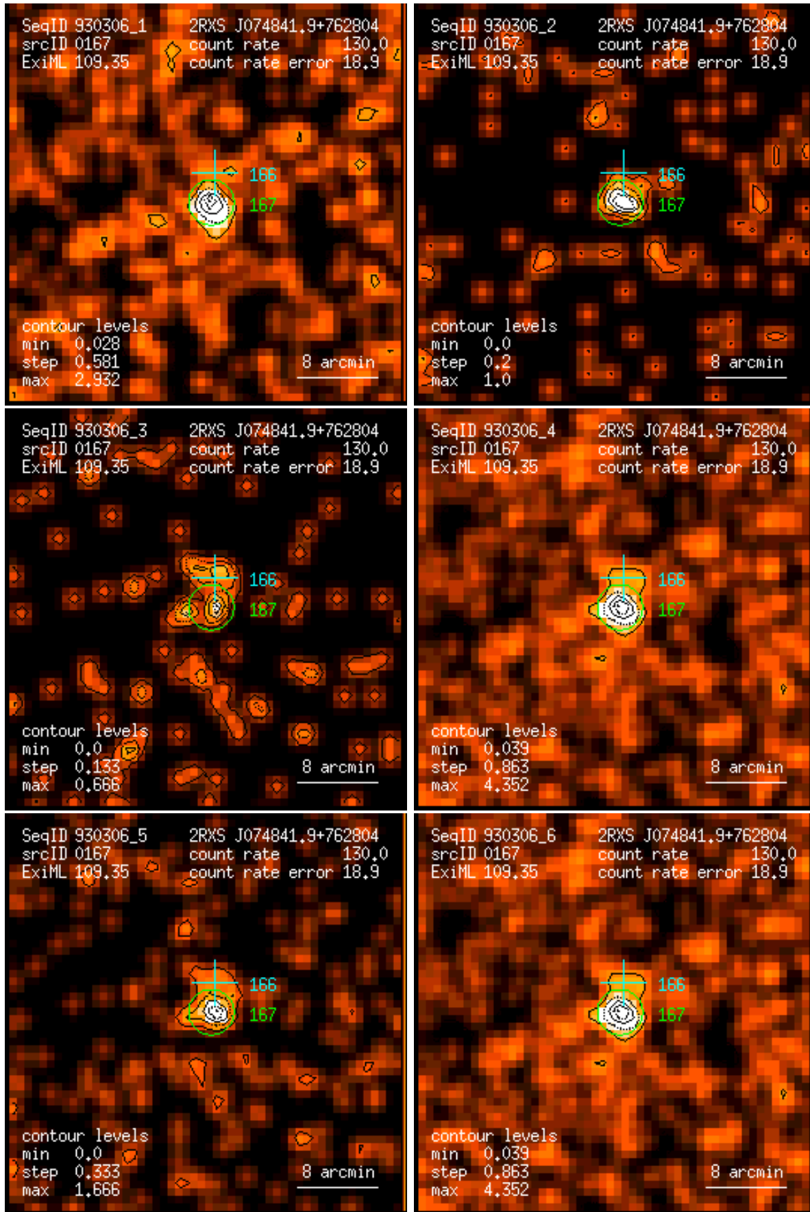
Figure 167: RASS 930306: detection 0167: band rate images, Gaussian filter: (1) PSPC channels 11 – 41, (2) 52 – 90, (3) 91 – 201, (4) 11 – 235, (5) 52 – 201, (6) 11 – 201. Broad band rates in counts/ks. Band rate contour levels in counts/ks/arcmin 2 .
