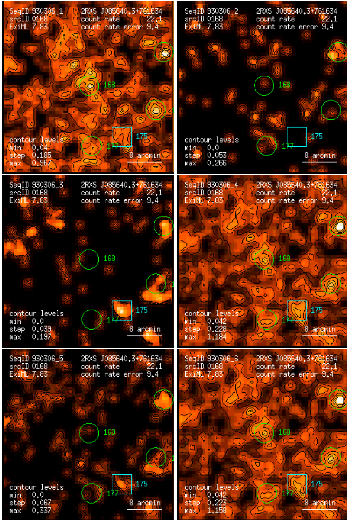
Figure 168: RASS 930306: detection 0168: band rate images, Gaussian filter: (1) PSPC channels 11 – 41, (2) 52 – 90, (3) 91 – 201, (4) 11 – 235, (5) 52 – 201, (6) 11 – 201. Broad band rates in counts/ks. Band rate contour levels in counts/ks/arcmin 2 .
