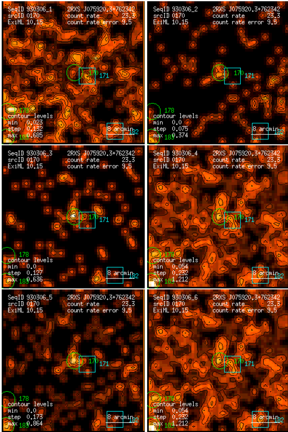
Figure 170: RASS 930306: detection 0170: band rate images, Gaussian filter: (1) PSPC channels 11 – 41, (2) 52 – 90, (3) 91 – 201, (4) 11 – 235, (5) 52 – 201, (6) 11 – 201. Broad band rates in counts/ks. Band rate contour levels in counts/ks/arcmin 2 .
