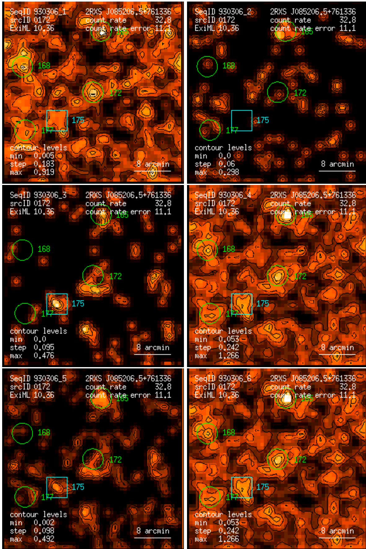
Figure 172: RASS 930306: detection 0172: band rate images, Gaussian filter: (1) PSPC channels 11 – 41, (2) 52 – 90, (3) 91 – 201, (4) 11 – 235, (5) 52 – 201, (6) 11 – 201. Broad band rates in counts/ks. Band rate contour levels in counts/ks/arcmin 2 .
