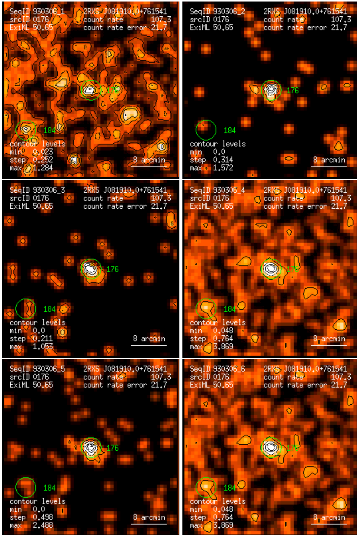
Figure 176: RASS 930306: detection 0176: band rate images, Gaussian filter: (1) PSPC channels 11 – 41, (2) 52 – 90, (3) 91 – 201, (4) 11 – 235, (5) 52 – 201, (6) 11 – 201. Broad band rates in counts/ks. Band rate contour levels in counts/ks/arcmin 2 .
