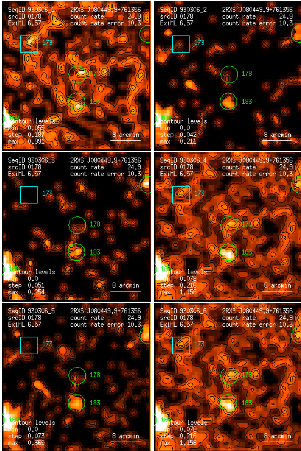
Figure 178: RASS 930306: detection 0178: band rate images, Gaussian filter: (1) PSPC channels 11 – 41, (2) 52 – 90, (3) 91 – 201, (4) 11 – 235, (5) 52 – 201, (6) 11 – 201. Broad band rates in counts/ks. Band rate contour levels in counts/ks/arcmin 2 .
