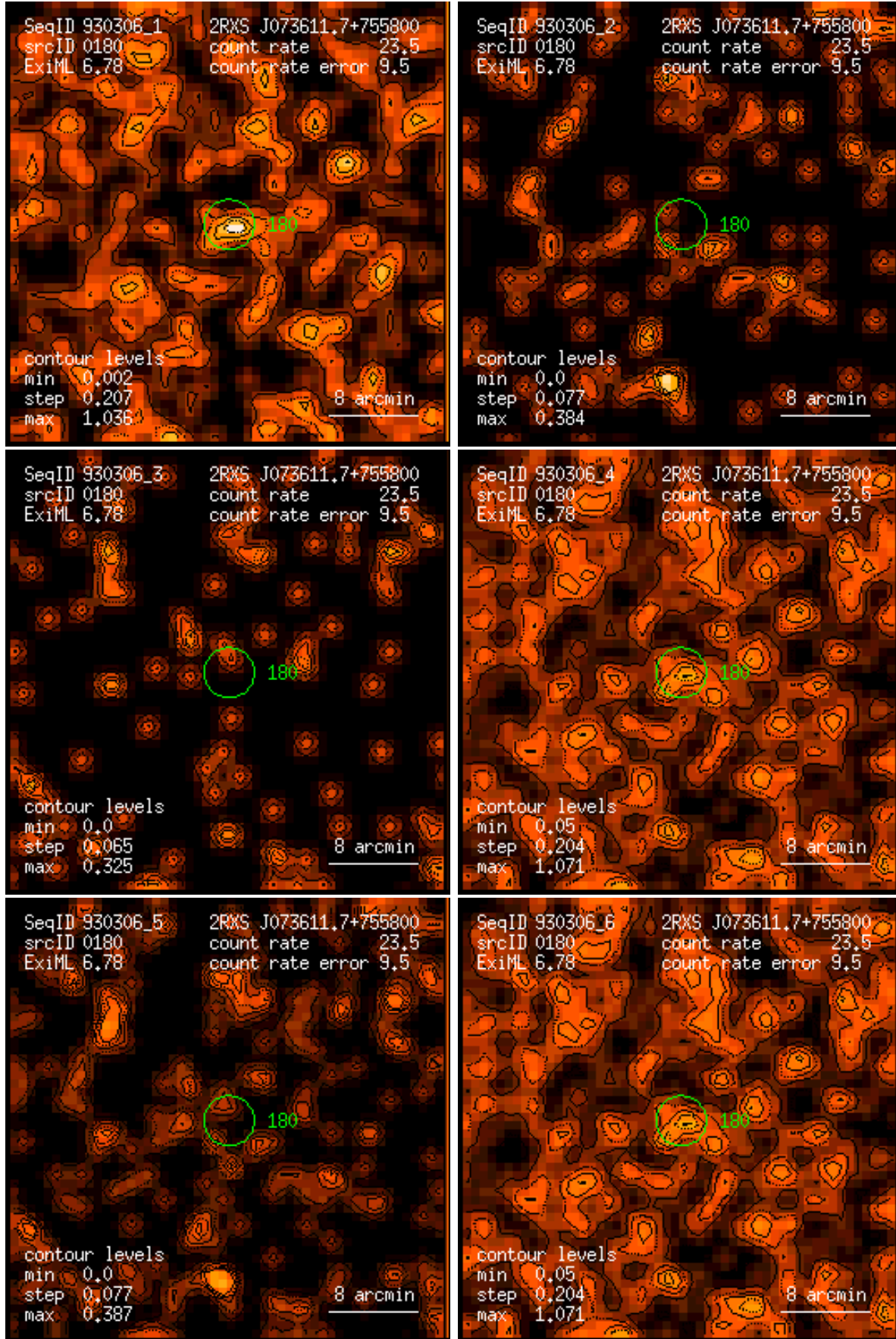
Figure 180: RASS 930306: detection 0180: band rate images, Gaussian filter: (1) PSPC channels 11 – 41, (2) 52 – 90, (3) 91 – 201, (4) 11 – 235, (5) 52 – 201, (6) 11 – 201. Broad band rates in counts/ks. Band rate contour levels in counts/ks/arcmin 2 .
