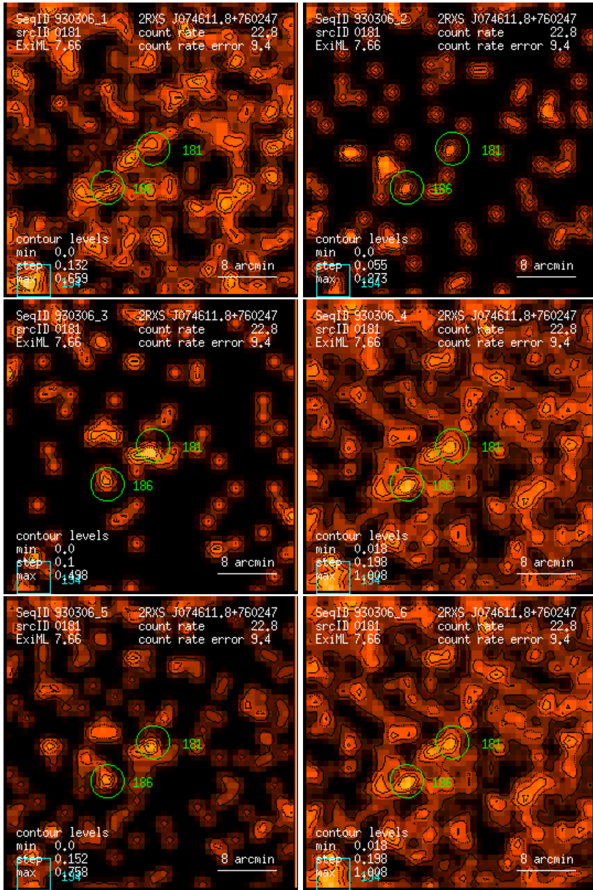
Figure 181: RASS 930306: detection 0181: band rate images, Gaussian filter: (1) PSPC channels 11 – 41, (2) 52 – 90, (3) 91 – 201, (4) 11 – 235, (5) 52 – 201, (6) 11 – 201. Broad band rates in counts/ks. Band rate contour levels in counts/ks/arcmin 2 .
