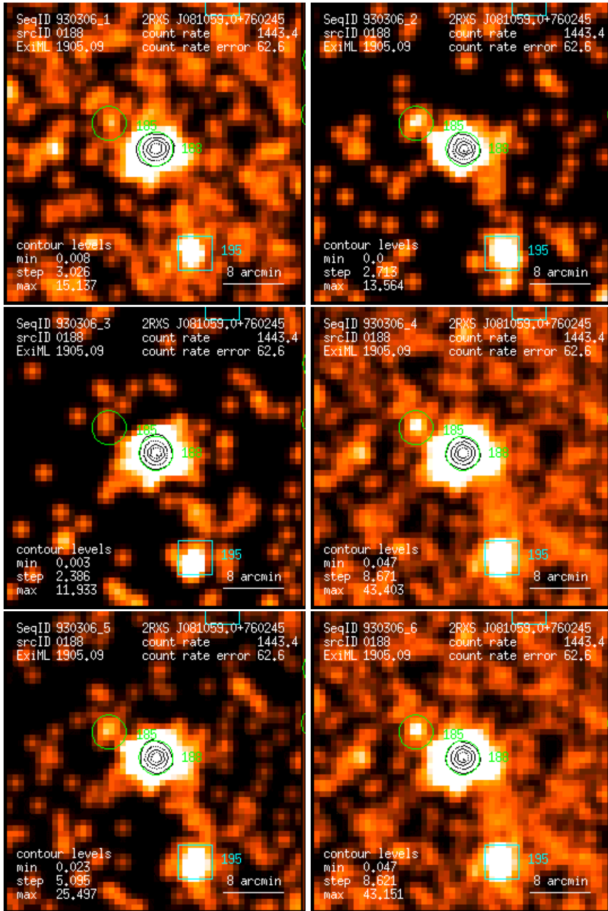
Figure 188: RASS 930306: detection 0188: band rate images, Gaussian filter: (1) PSPC channels 11 – 41, (2) 52 – 90, (3) 91 – 201, (4) 11 – 235, (5) 52 – 201, (6) 11 – 201. Broad band rates in counts/ks. Band rate contour levels in counts/ks/arcmin 2 .
