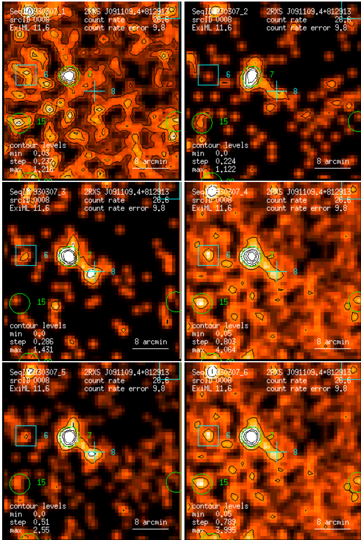
Figure 8: RASS 930307: detection 0008: band rate images, Gaussian filter: (1) PSPC channels 11 – 41, (2) 52 – 90, (3) 91 – 201, (4) 11 – 235, (5) 52 – 201, (6) 11 – 201. Broad band rates in counts/ks. Band rate contour levels in counts/ks/arcmin 2 .
