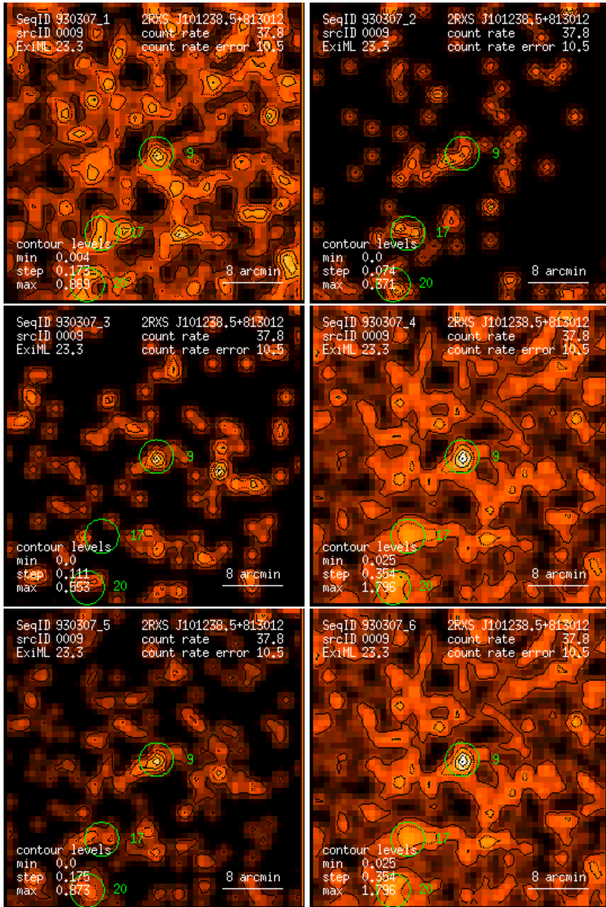
Figure 9: RASS 930307: detection 0009: band rate images, Gaussian filter: (1) PSPC channels 11 – 41, (2) 52 – 90, (3) 91 – 201, (4) 11 – 235, (5) 52 – 201, (6) 11 – 201. Broad band rates in counts/ks. Band rate contour levels in counts/ks/arcmin 2 .
