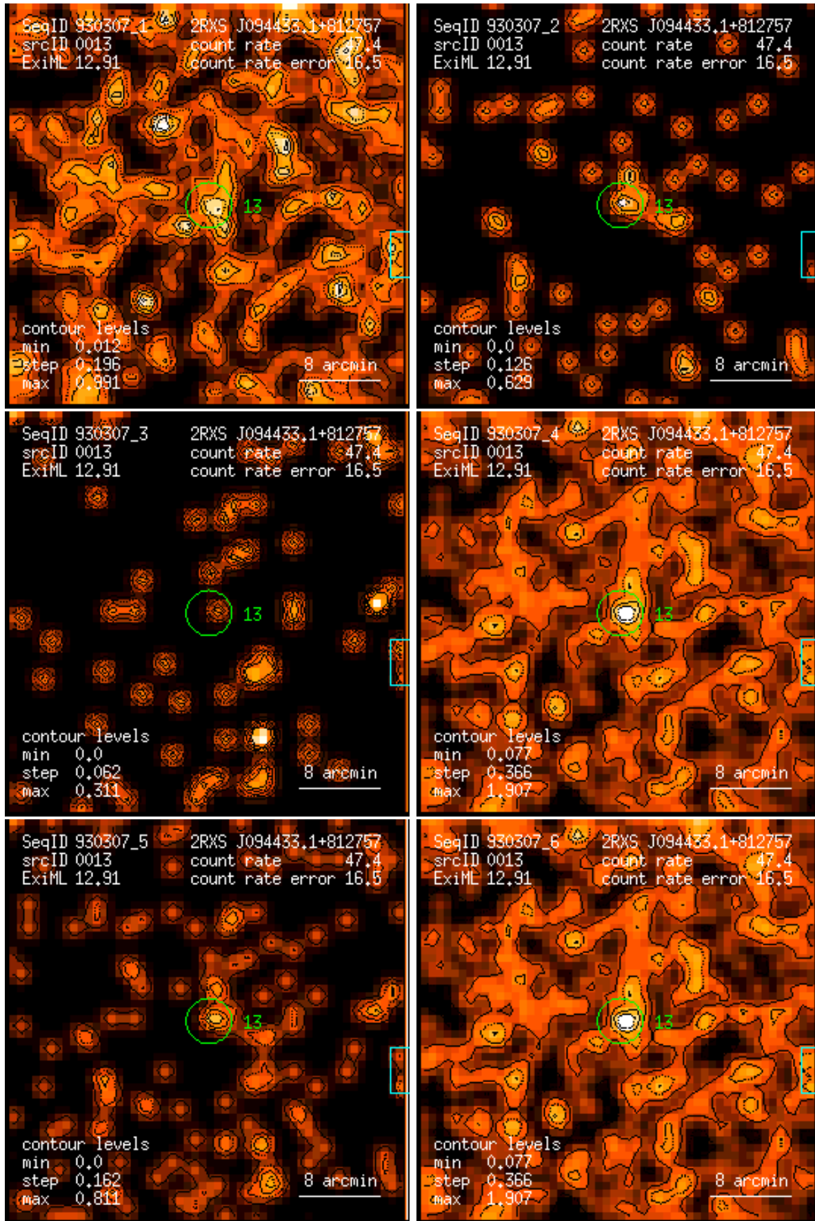
Figure 13: RASS 930307: detection 0013: band rate images, Gaussian filter: (1) PSPC channels 11 – 41, (2) 52 – 90, (3) 91 – 201, (4) 11 – 235, (5) 52 – 201, (6) 11 – 201. Broad band rates in counts/ks. Band rate contour levels in counts/ks/arcmin 2 .
