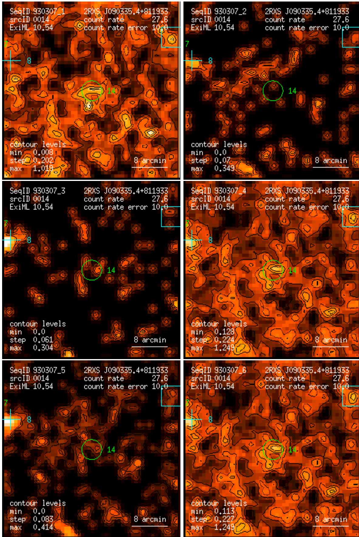
Figure 14: RASS 930307: detection 0014: band rate images, Gaussian filter: (1) PSPC channels 11 – 41, (2) 52 – 90, (3) 91 – 201, (4) 11 – 235, (5) 52 – 201, (6) 11 – 201. Broad band rates in counts/ks. Band rate contour levels in counts/ks/arcmin 2 .
