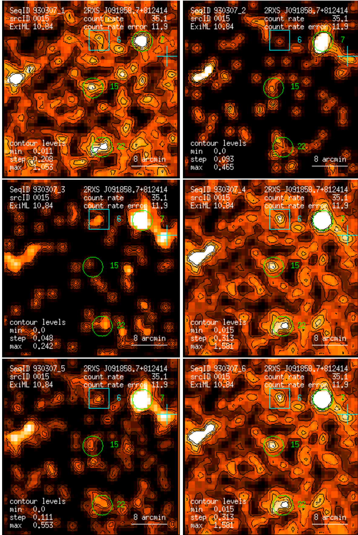
Figure 15: RASS 930307: detection 0015: band rate images, Gaussian filter: (1) PSPC channels 11 – 41, (2) 52 – 90, (3) 91 – 201, (4) 11 – 235, (5) 52 – 201, (6) 11 – 201. Broad band rates in counts/ks. Band rate contour levels in counts/ks/arcmin 2 .
