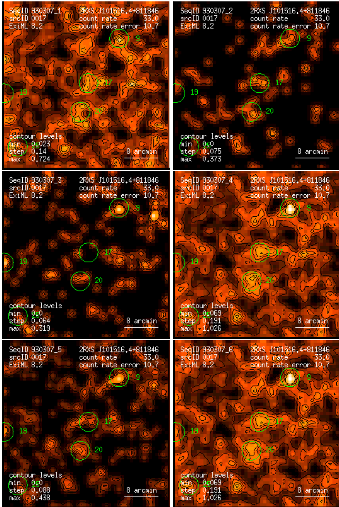
Figure 17: RASS 930307: detection 0017: band rate images, Gaussian filter: (1) PSPC channels 11 – 41, (2) 52 – 90, (3) 91 – 201, (4) 11 – 235, (5) 52 – 201, (6) 11 – 201. Broad band rates in counts/ks. Band rate contour levels in counts/ks/arcmin 2 .
