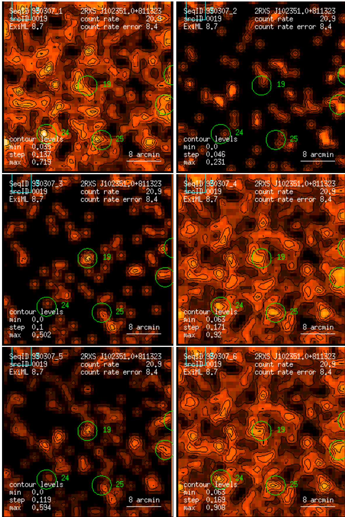
Figure 19: RASS 930307: detection 0019: band rate images, Gaussian filter: (1) PSPC channels 11 – 41, (2) 52 – 90, (3) 91 – 201, (4) 11 – 235, (5) 52 – 201, (6) 11 – 201. Broad band rates in counts/ks. Band rate contour levels in counts/ks/arcmin 2 .
