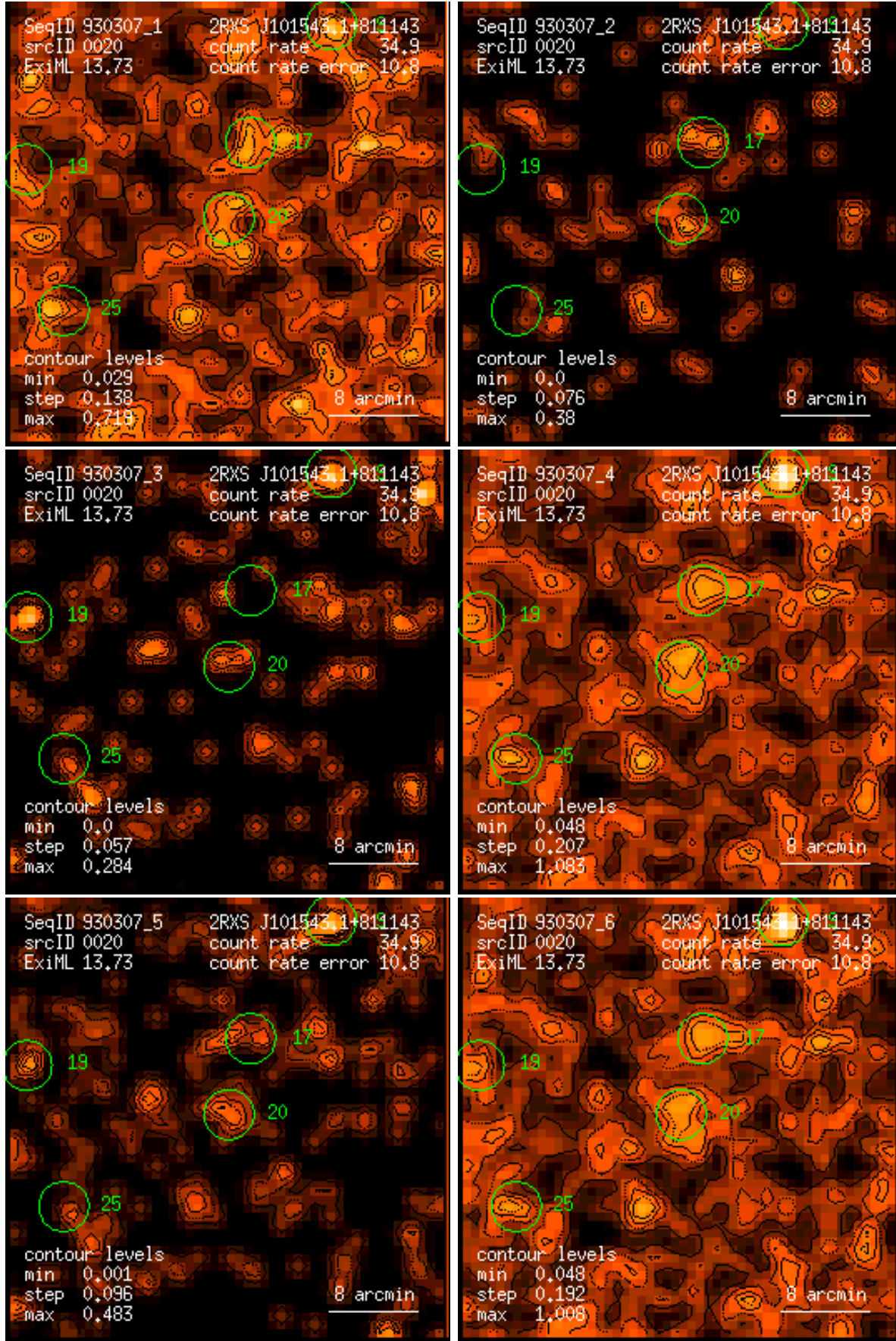
Figure 20: RASS 930307: detection 0020: band rate images, Gaussian filter: (1) PSPC channels 11 – 41, (2) 52 – 90, (3) 91 – 201, (4) 11 – 235, (5) 52 – 201, (6) 11 – 201. Broad band rates in counts/ks. Band rate contour levels in counts/ks/arcmin 2 .
