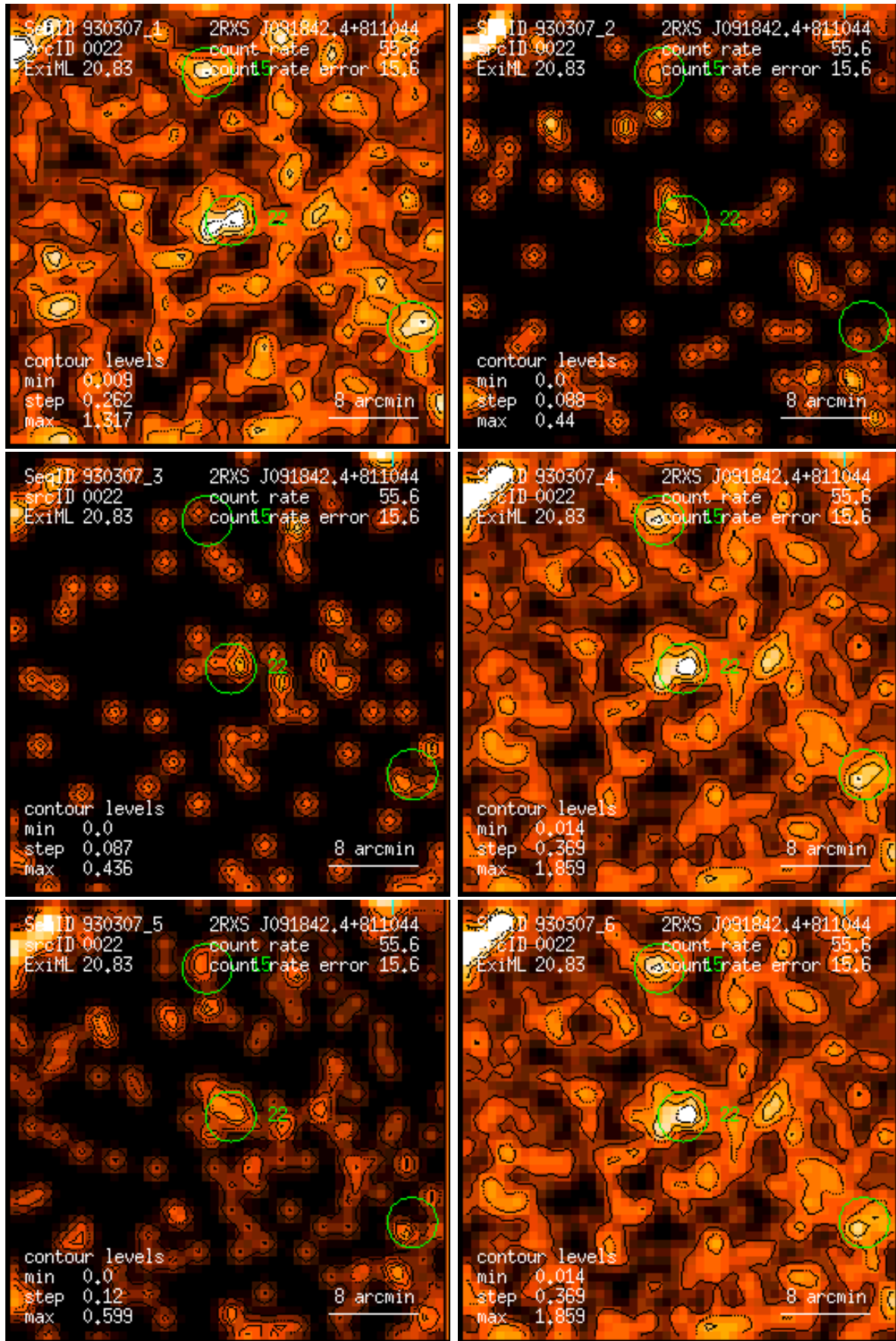
Figure 22: RASS 930307: detection 0022: band rate images, Gaussian filter: (1) PSPC channels 11 – 41, (2) 52 – 90, (3) 91 – 201, (4) 11 – 235, (5) 52 – 201, (6) 11 – 201. Broad band rates in counts/ks. Band rate contour levels in counts/ks/arcmin 2 .
