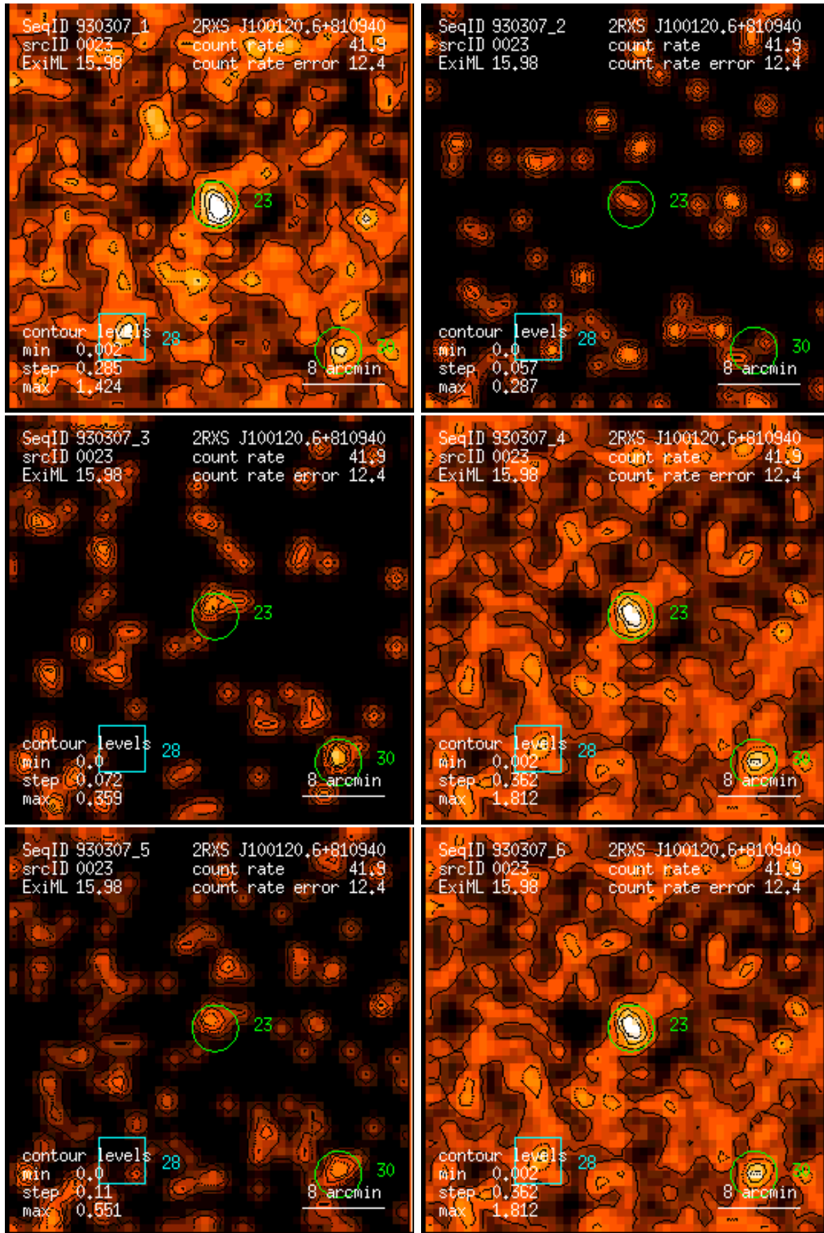
Figure 23: RASS 930307: detection 0023: band rate images, Gaussian filter: (1) PSPC channels 11 – 41, (2) 52 – 90, (3) 91 – 201, (4) 11 – 235, (5) 52 – 201, (6) 11 – 201. Broad band rates in counts/ks. Band rate contour levels in counts/ks/arcmin 2 .
