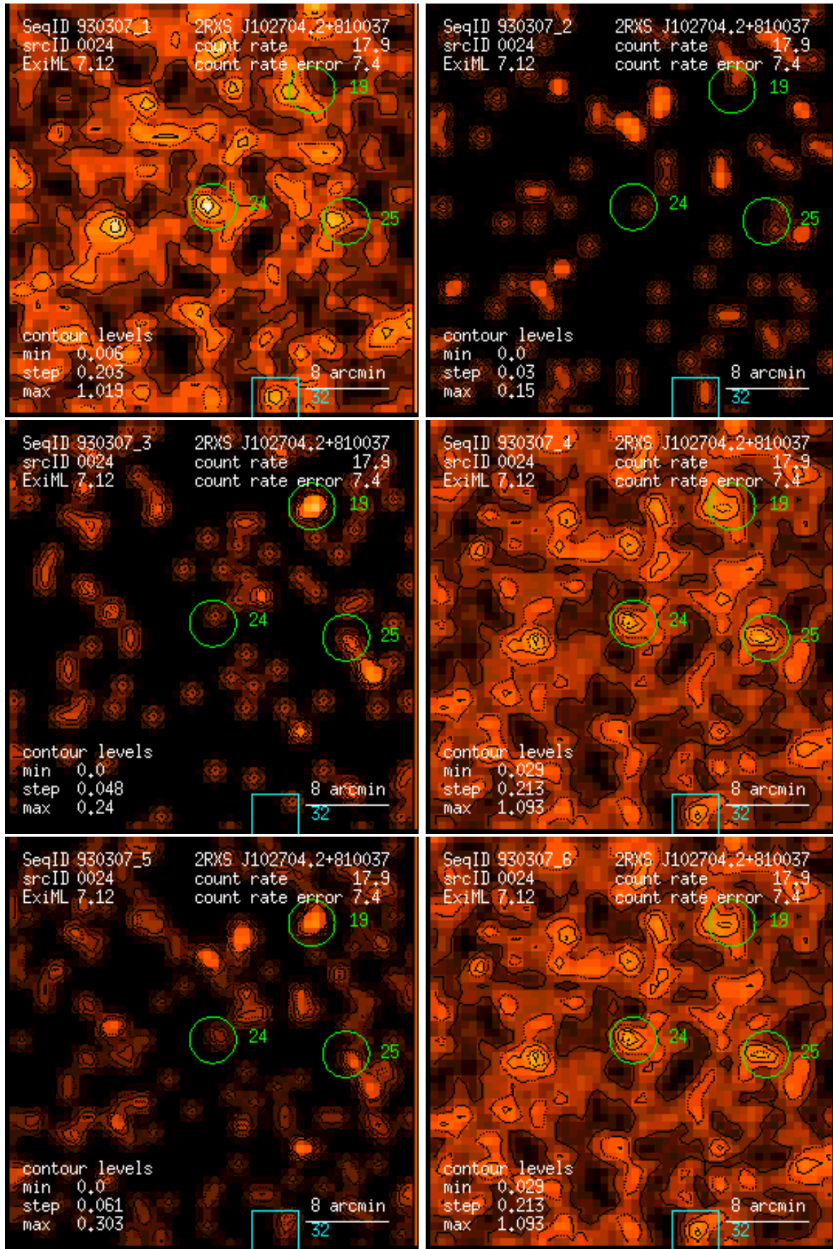
Figure 24: RASS 930307: detection 0024: band rate images, Gaussian filter: (1) PSPC channels 11 – 41, (2) 52 – 90, (3) 91 – 201, (4) 11 – 235, (5) 52 – 201, (6) 11 – 201. Broad band rates in counts/ks. Band rate contour levels in counts/ks/arcmin 2 .
