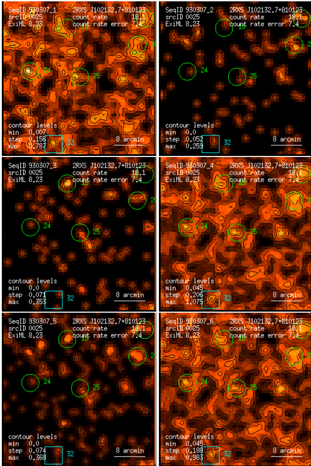
Figure 25: RASS 930307: detection 0025: band rate images, Gaussian filter: (1) PSPC channels 11 – 41, (2) 52 – 90, (3) 91 – 201, (4) 11 – 235, (5) 52 – 201, (6) 11 – 201. Broad band rates in counts/ks. Band rate contour levels in counts/ks/arcmin 2 .
