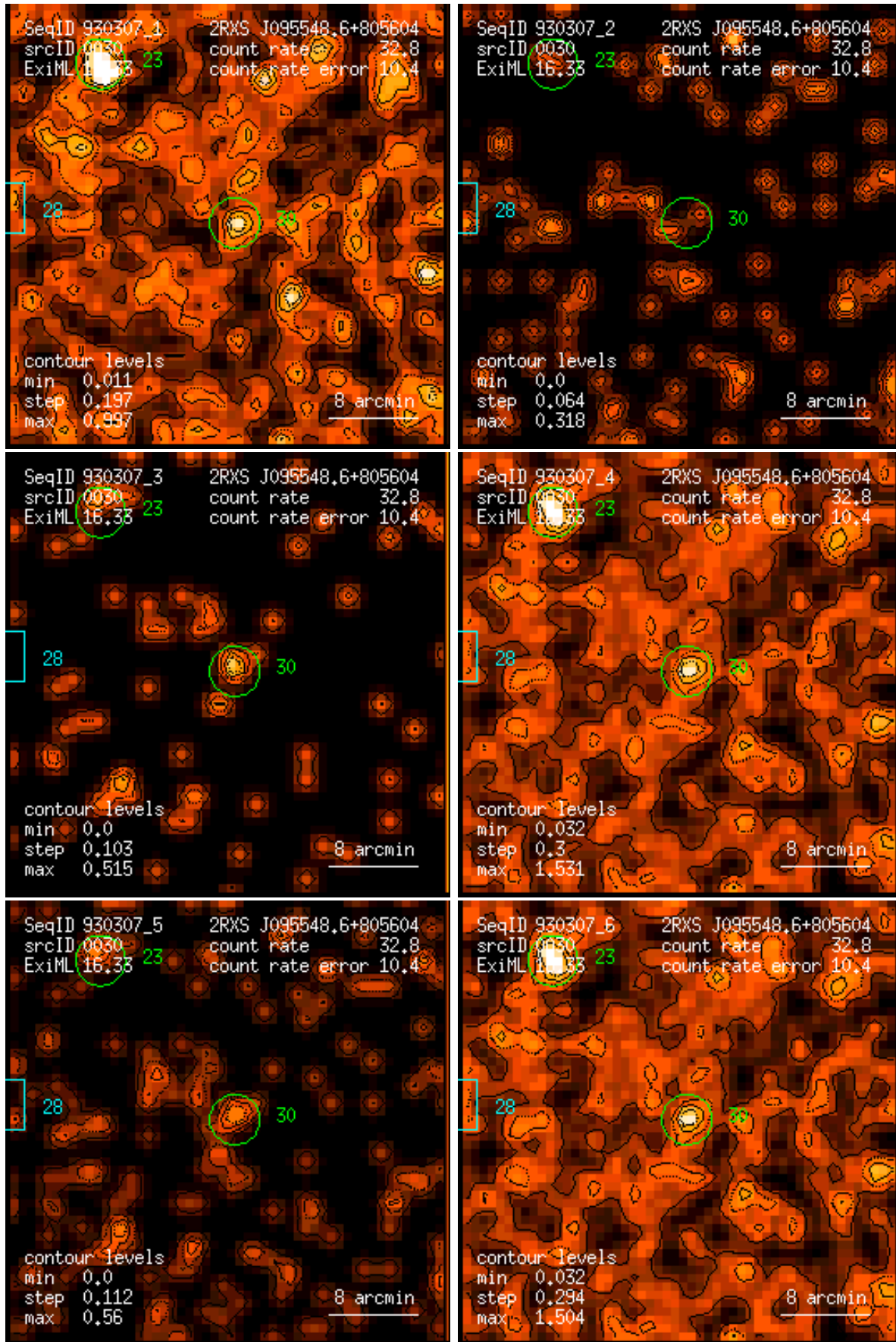
Figure 30: RASS 930307: detection 0030: band rate images, Gaussian filter: (1) PSPC channels 11 – 41, (2) 52 – 90, (3) 91 – 201, (4) 11 – 235, (5) 52 – 201, (6) 11 – 201. Broad band rates in counts/ks. Band rate contour levels in counts/ks/arcmin 2 .
