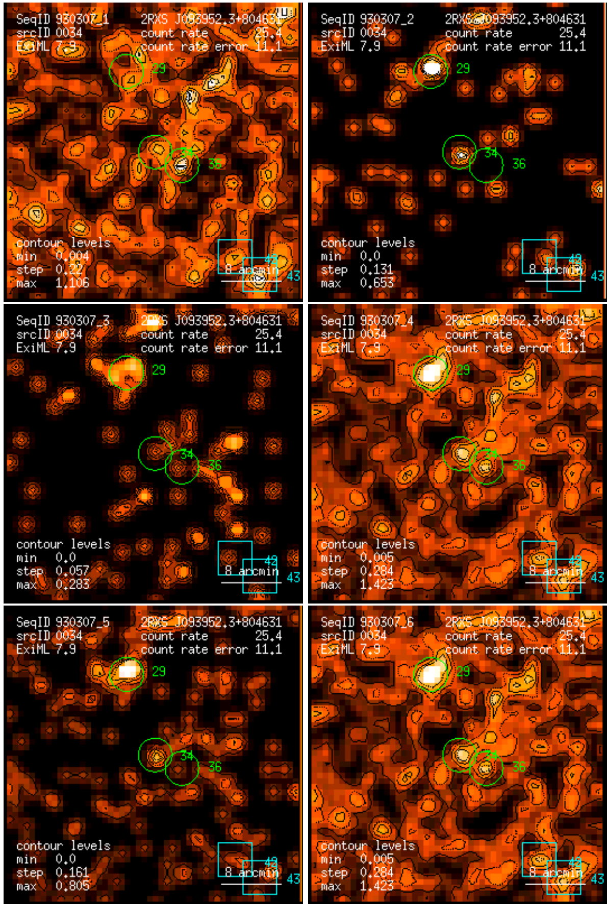
Figure 34: RASS 930307: detection 0034: band rate images, Gaussian filter: (1) PSPC channels 11 – 41, (2) 52 – 90, (3) 91 – 201, (4) 11 – 235, (5) 52 – 201, (6) 11 – 201. Broad band rates in counts/ks. Band rate contour levels in counts/ks/arcmin 2 .
