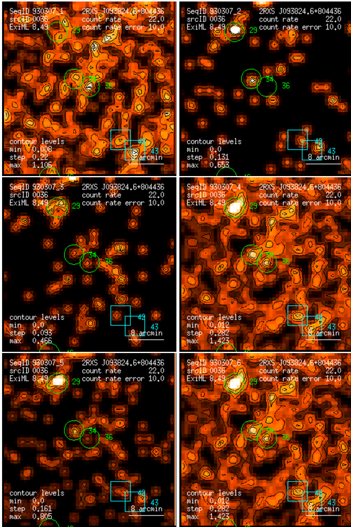
Figure 36: RASS 930307: detection 0036: band rate images, Gaussian filter: (1) PSPC channels 11 – 41, (2) 52 – 90, (3) 91 – 201, (4) 11 – 235, (5) 52 – 201, (6) 11 – 201. Broad band rates in counts/ks. Band rate contour levels in counts/ks/arcmin 2 .
