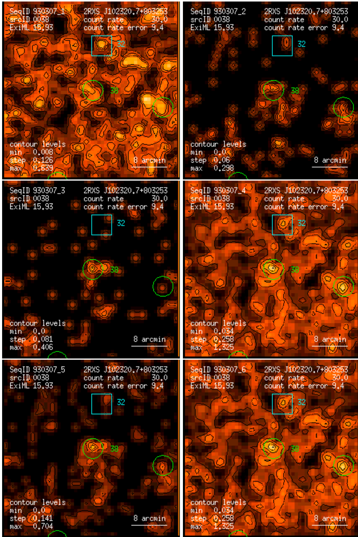
Figure 38: RASS 930307: detection 0038: band rate images, Gaussian filter: (1) PSPC channels 11 – 41, (2) 52 – 90, (3) 91 – 201, (4) 11 – 235, (5) 52 – 201, (6) 11 – 201. Broad band rates in counts/ks. Band rate contour levels in counts/ks/arcmin 2 .
