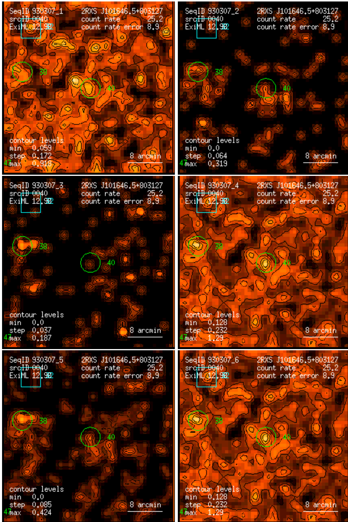
Figure 40: RASS 930307: detection 0040: band rate images, Gaussian filter: (1) PSPC channels 11 – 41, (2) 52 – 90, (3) 91 – 201, (4) 11 – 235, (5) 52 – 201, (6) 11 – 201. Broad band rates in counts/ks. Band rate contour levels in counts/ks/arcmin 2 .
