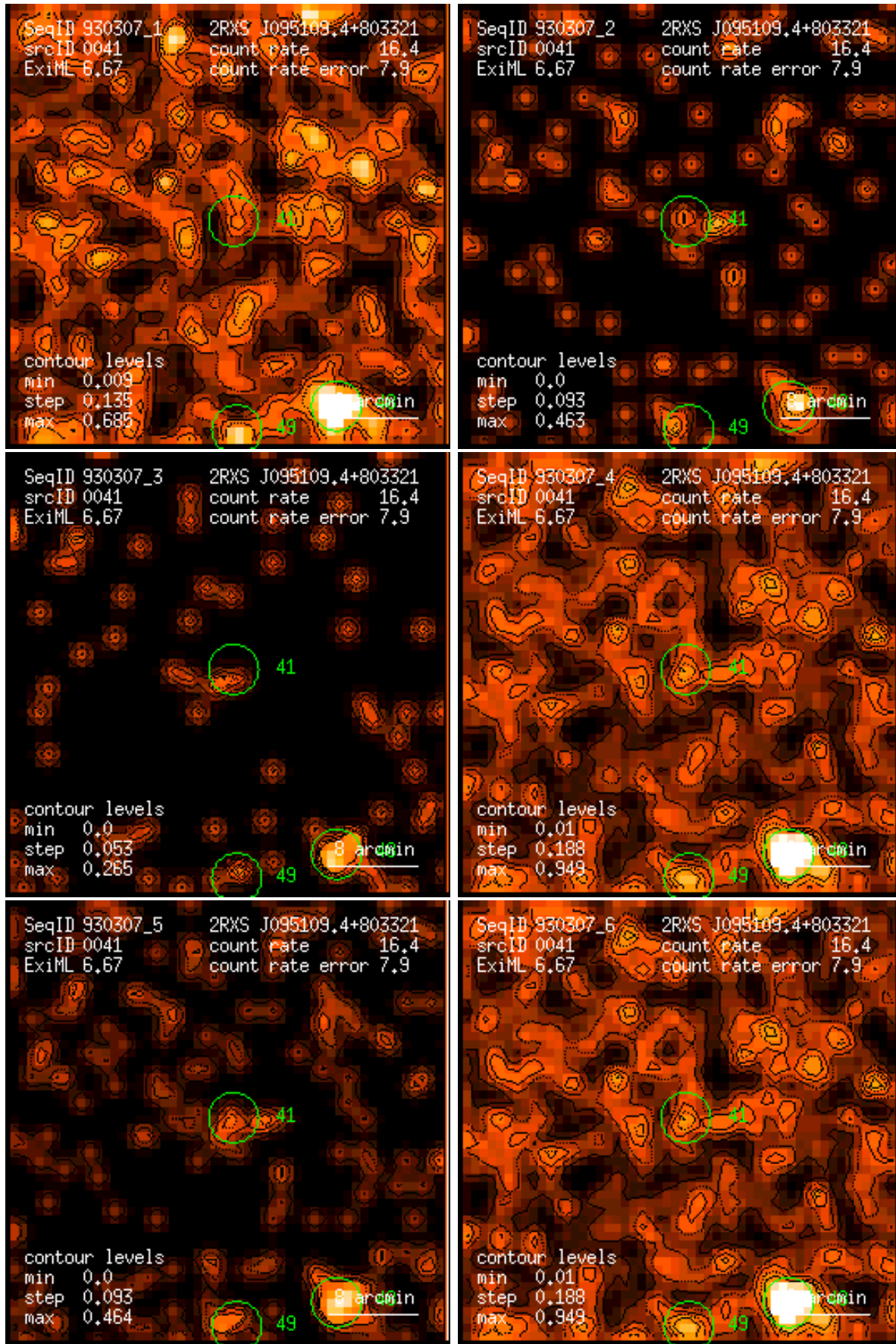
Figure 41: RASS 930307: detection 0041: band rate images, Gaussian filter: (1) PSPC channels 11 – 41, (2) 52 – 90, (3) 91 – 201, (4) 11 – 235, (5) 52 – 201, (6) 11 – 201. Broad band rates in counts/ks. Band rate contour levels in counts/ks/arcmin 2 .
