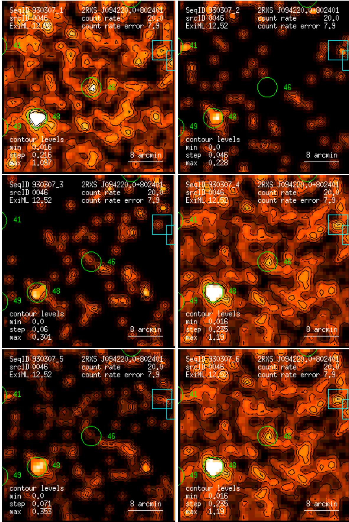
Figure 46: RASS 930307: detection 0046: band rate images, Gaussian filter: (1) PSPC channels 11 – 41, (2) 52 – 90, (3) 91 – 201, (4) 11 – 235, (5) 52 – 201, (6) 11 – 201. Broad band rates in counts/ks. Band rate contour levels in counts/ks/arcmin 2 .
